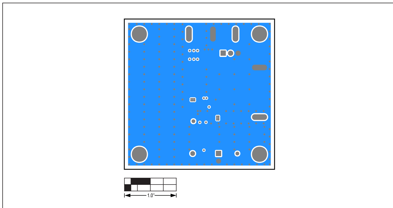
MAXM15062 EV Kit PCB Layout—Bottom Layer
