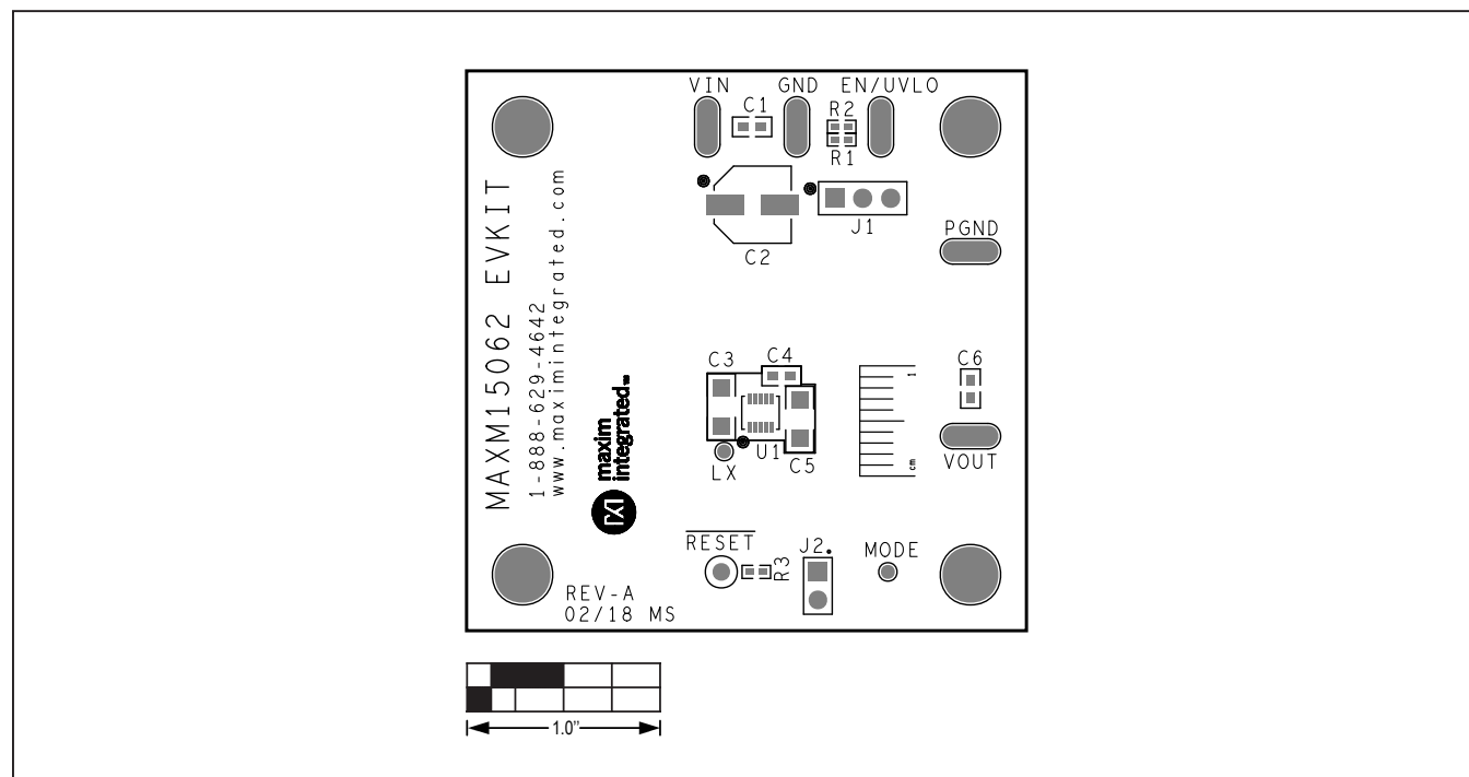
MAXM15062 EV Kit PCB Layout—Silk Top
