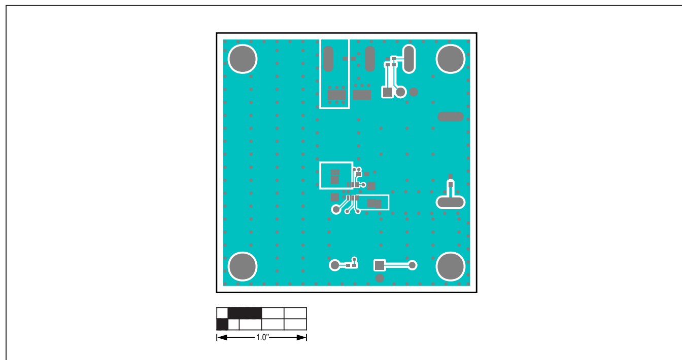
MAXM15062 EV Kit PCB Layout—Top Layer
